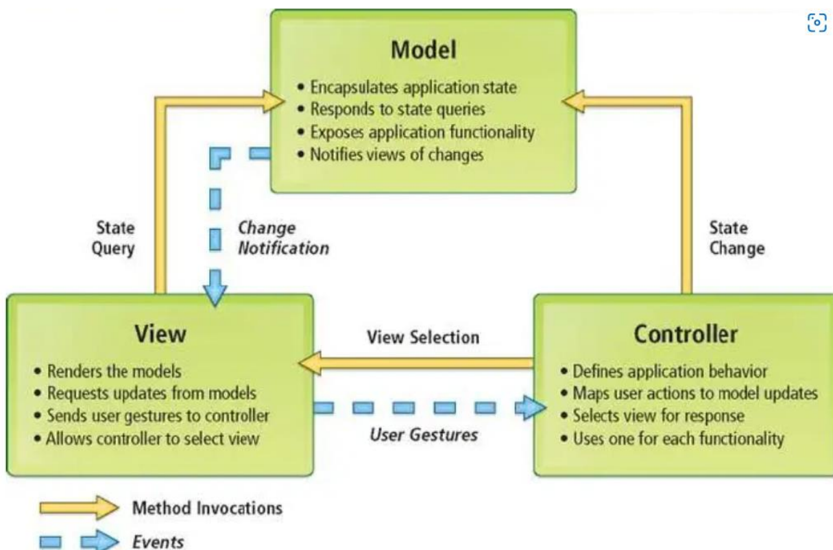
MVC (Model View Controller Flow) Diagram
